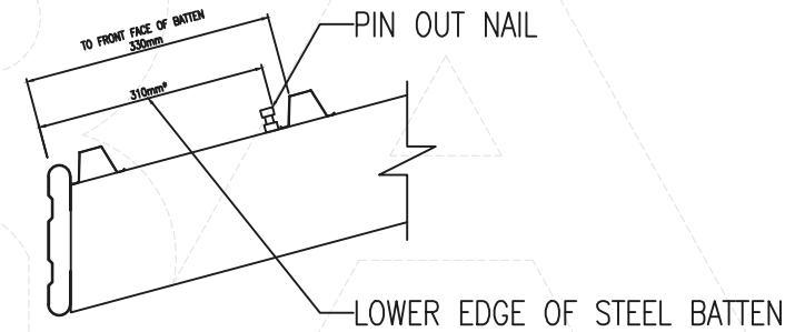
EAVE AND FIRST BATTEN LOCATION/SPACING
