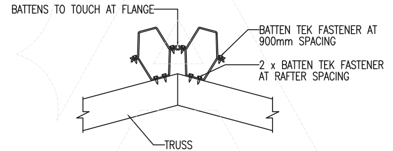
RIDGE BATTEN INSTALLATION
