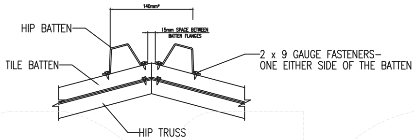
BARREL – HIP BATTEN INSTALLATION
