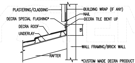
METHOD (v) DECRA FLASHING INSTALLATION AT VERTICAL WALL JOINT
