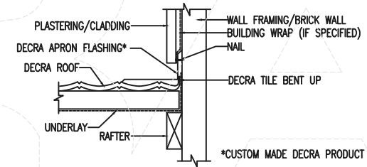
METHOD (iv) DECRA FLASHING INSTALLATION AT VERTICAL WALL JOINT
