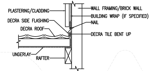
METHOD (iii) DECRA FLASHING INSTALLATION AT VERTICAL WALL JOINT
