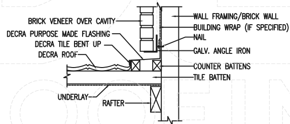
METHOD (ii) DECRA FLASHING INSTALLATION AT VERTICAL WALL JOINT
