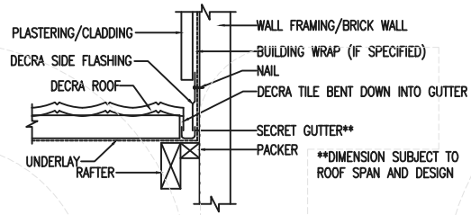
METHOD (i) DECRA FLASHING INSTALLATION AT VERTICAL WALL JOINT
